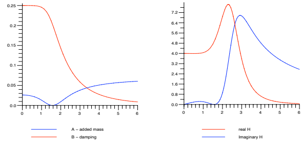
Added Mass and Damping and resulting governing transfer function
